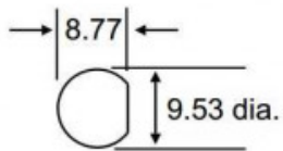
Panel Cutout 3/8"-27 Bushing
